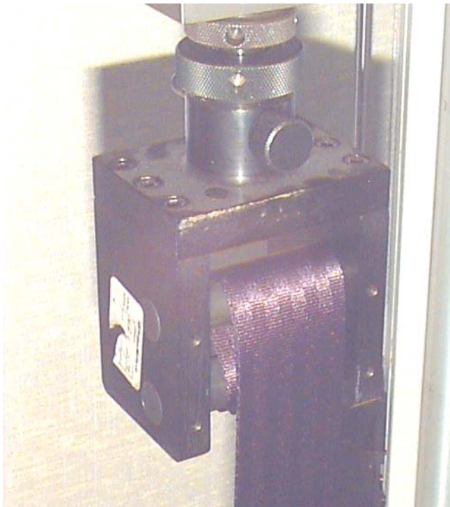
View of top HT43 belt grip attachment
