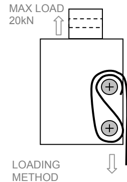
View of HT43 grips assembled with belt specimen and ready for test on H25KS machine
